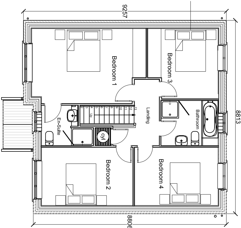
PROPOSED FIRST FLOOR PLAN SCALE 1:100 @ A3
